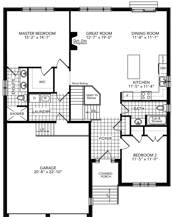
MAIN FLOOR
