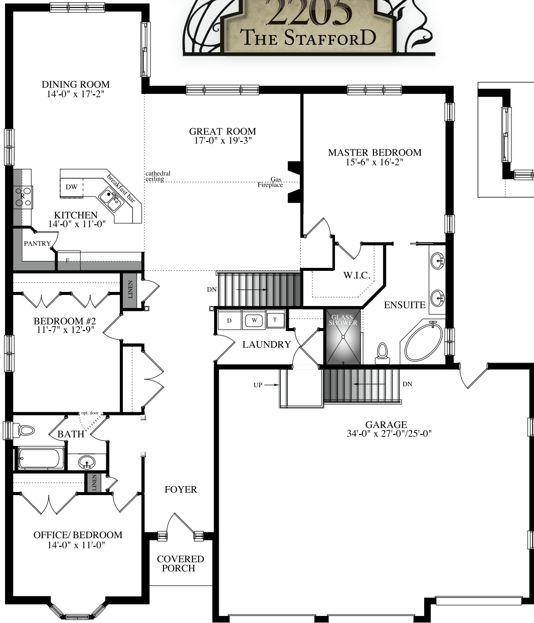
MAIN FLOOR
